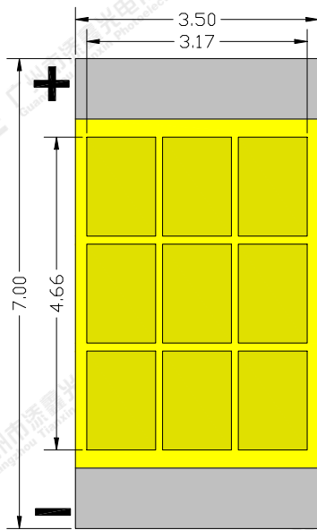
Top view
