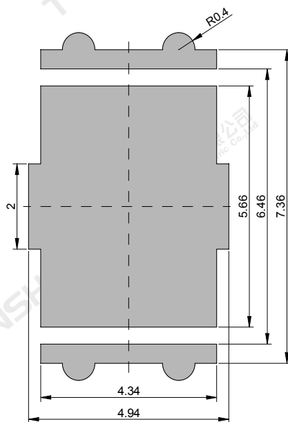
Recommended solder pad
