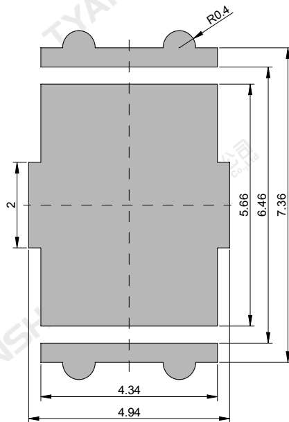
Recommended solder pad
