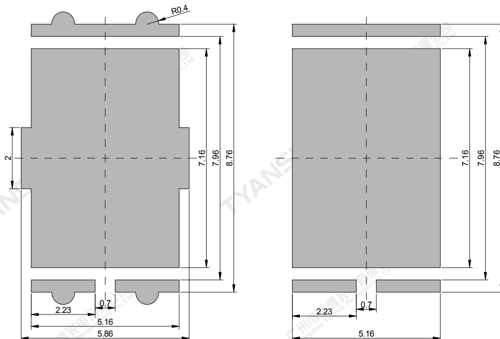
Recommended solder pad
