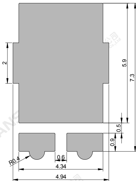
Recommended solder pad
