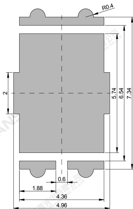
Recommended solder pad
