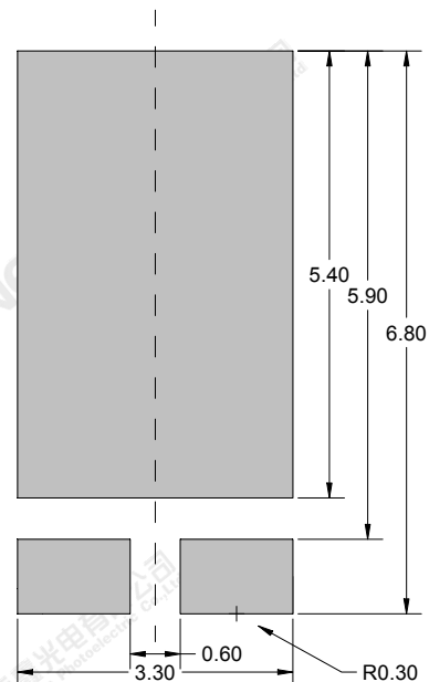
recommended stencil pattern
