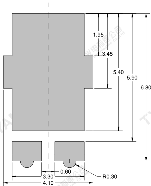
Recommended solder pad
